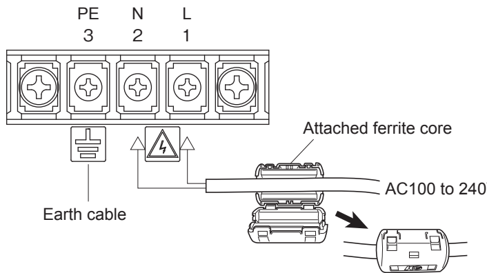
<Terminal block for power supply>
